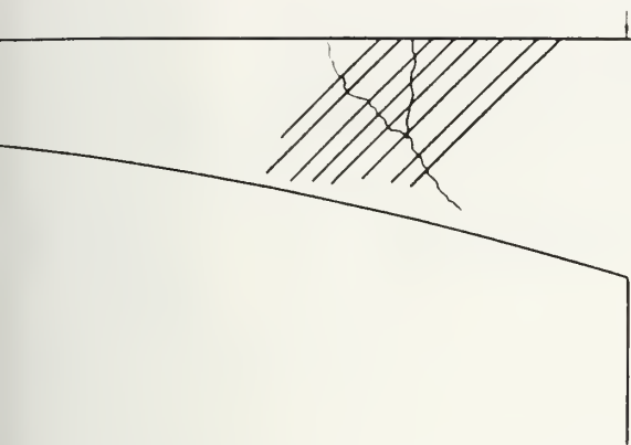
3.3—Reinforcing bar orientation used to effect the re- (Reference 43)
